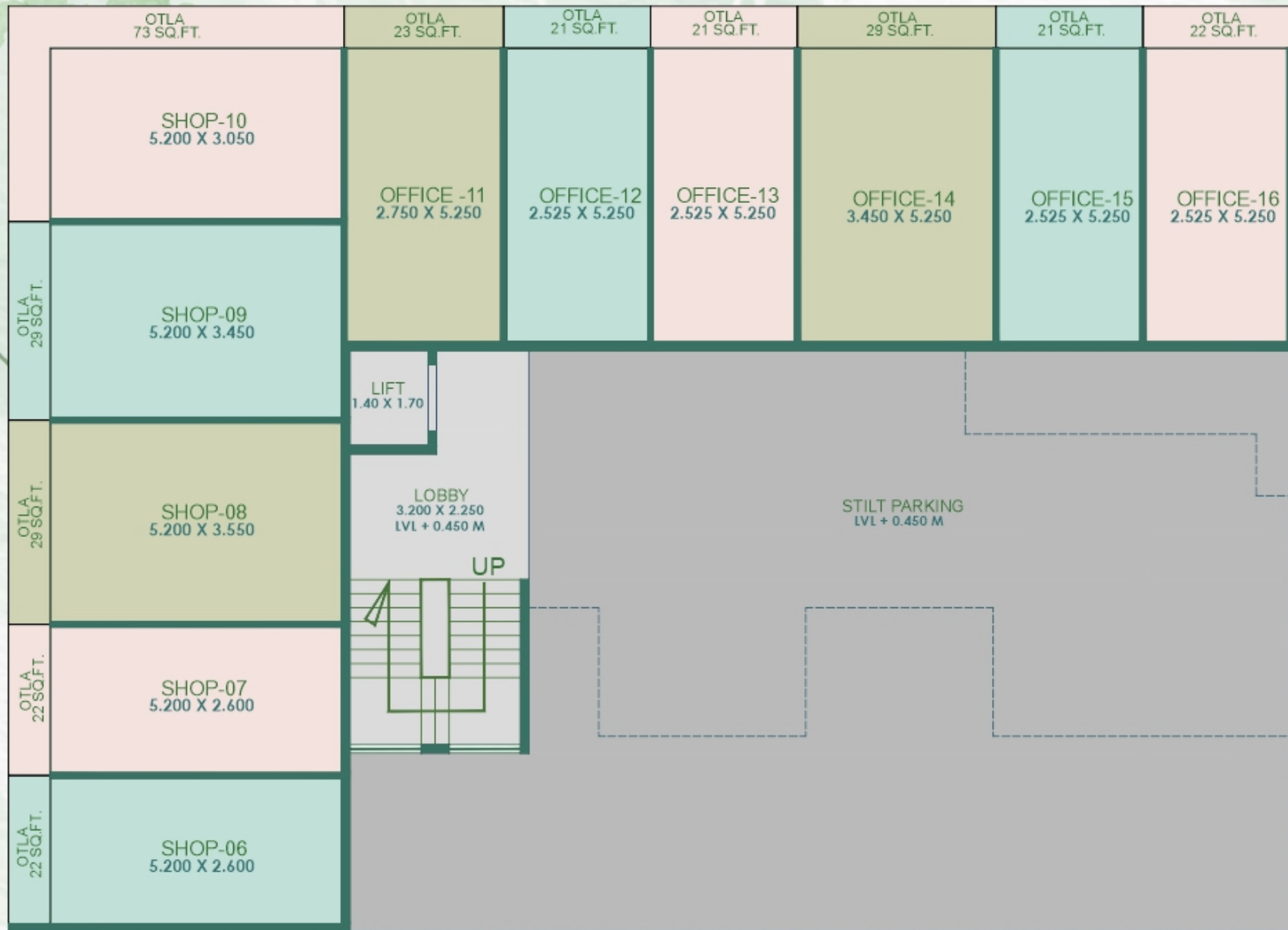
WING-D GROUND FLOOR PLAN
